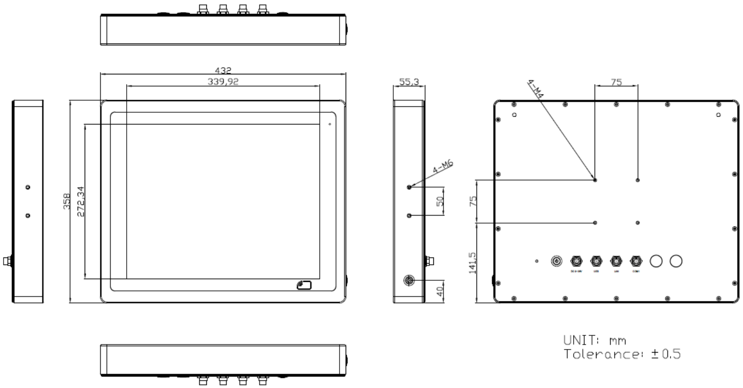
Figure 1.3: Dimensions of VITAM-917AP/R/G(H)
