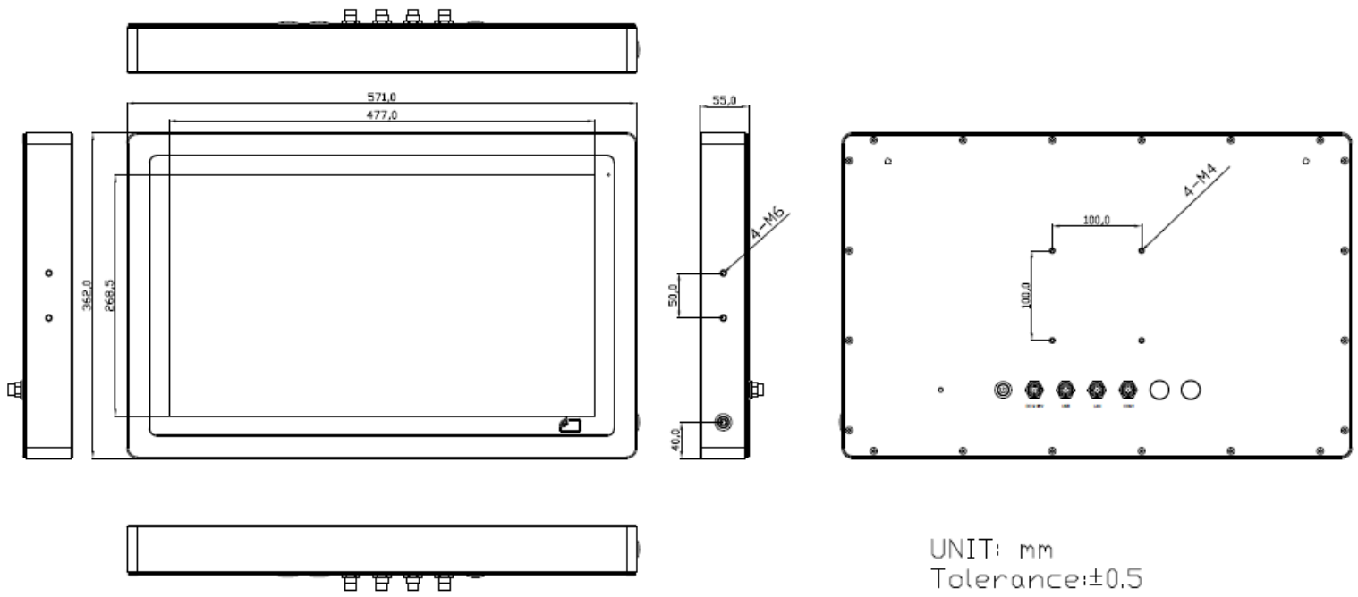
Figure 1.5: Dimensions of VITAM-921AP/R/G(H)
