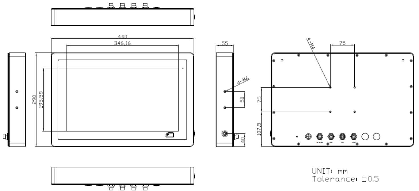
Figure 1.2: Dimensions of VITAM-916AP/R/G(H)
