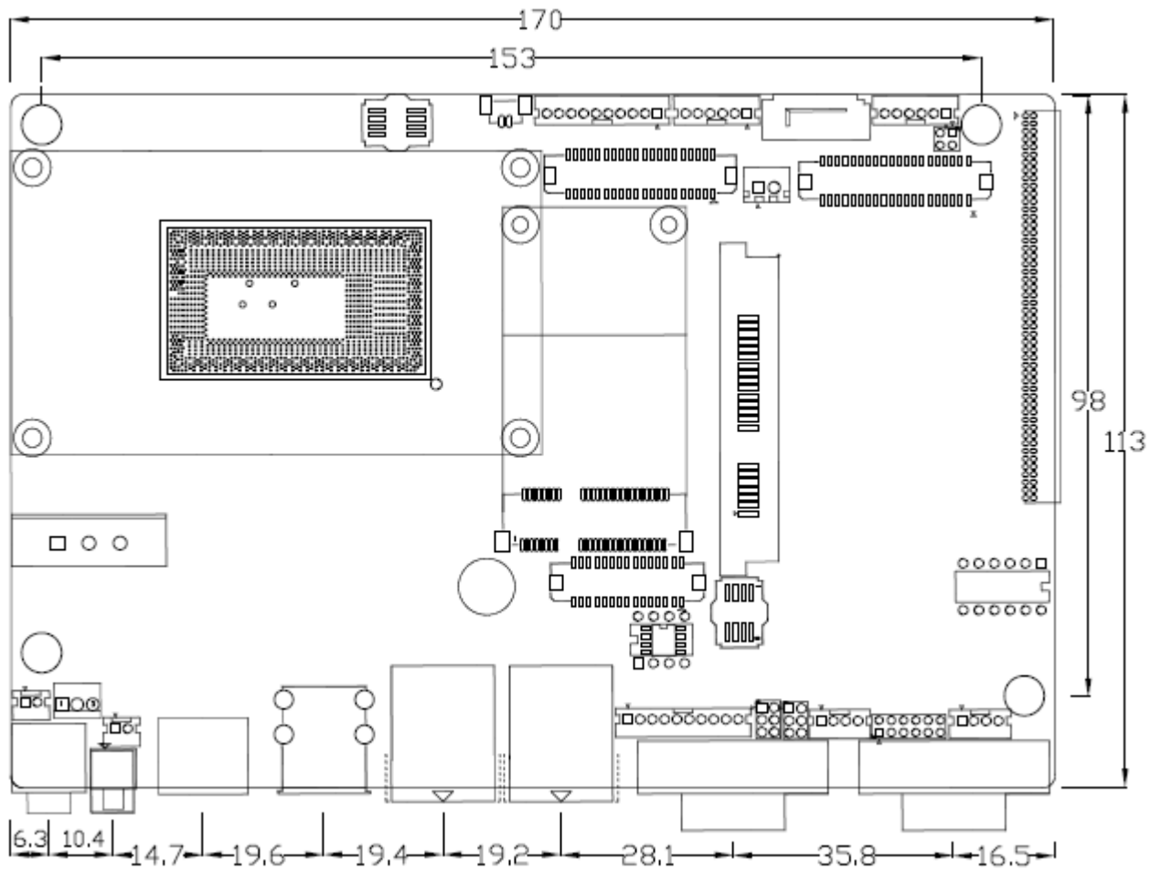
Figure 2.1: Motherboard Dimensions
